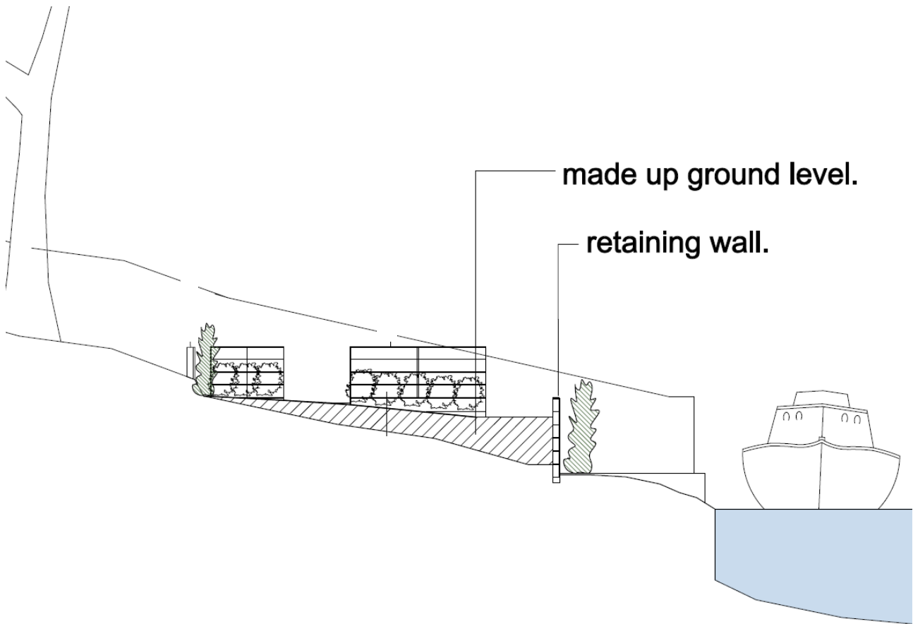
Appendix. 4 – Indicative Section through Site (retaining structure reduced in height to that shown and varies across its length)
